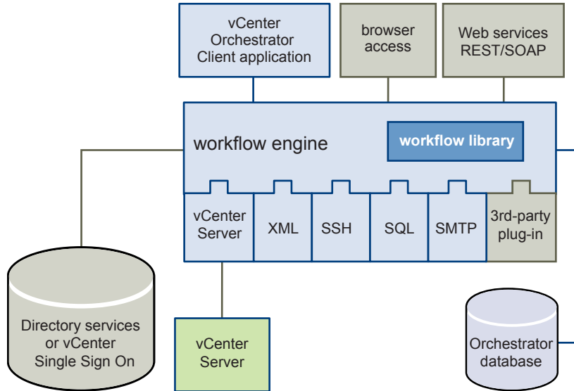
Figure 2-1. VMware vCenter Orchestrator Architecture
